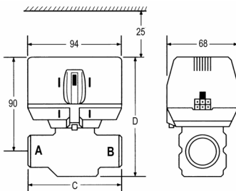
Fig. 1: Dimensions (mm)
