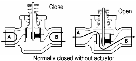
Fig. 2: Flow direction
